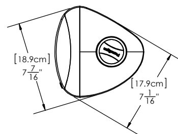
SPEAKER WITHOUT MOUNTING BRACKET
