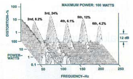
Fig. 7—Harmonic distortion for E_1 (41.2 Hz).
