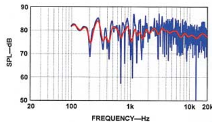
Fig. 6—Three-meter room response.
