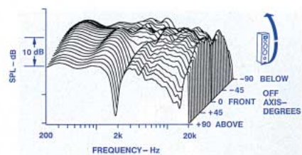
Fig. 4—Vertical off-axis frequency responses.
