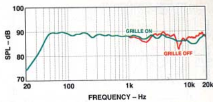
Fig. 1—One-meter, on-axis frequency response.
