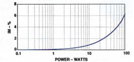
Fig. 8—IM distortion for A_4 (440 Hz) and E_1 (41.2 Hz) tones of equal power
