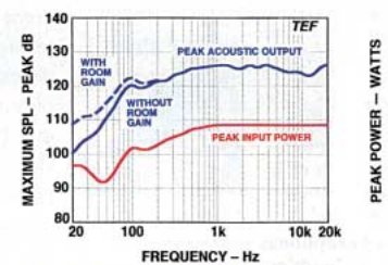
Fig. 9—Maximum peak input power and sound output.
