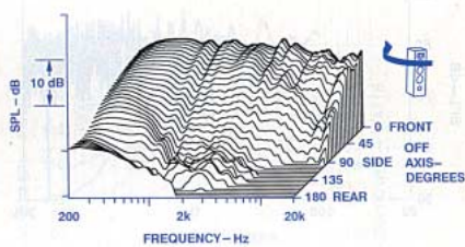
Fig. 3—Horizontal off-axis frequency response.
