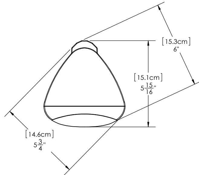
TOP VIEW WITH MOUNTING BRACKET
